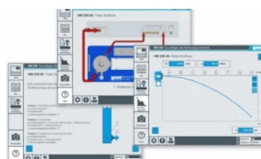
Software
